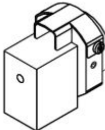
Welding shoe blank complete 50x30x38mm for FUSION 2 118.094
